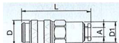
push-in
